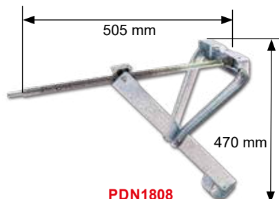
STANDARD 800 KG CORTO SHORT STANDARD 800 KG
